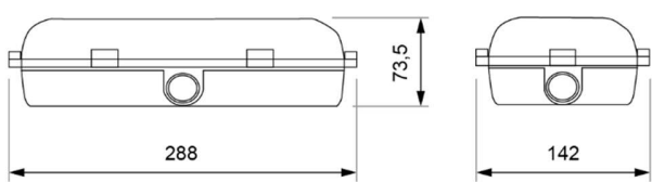
Watertight mounting
